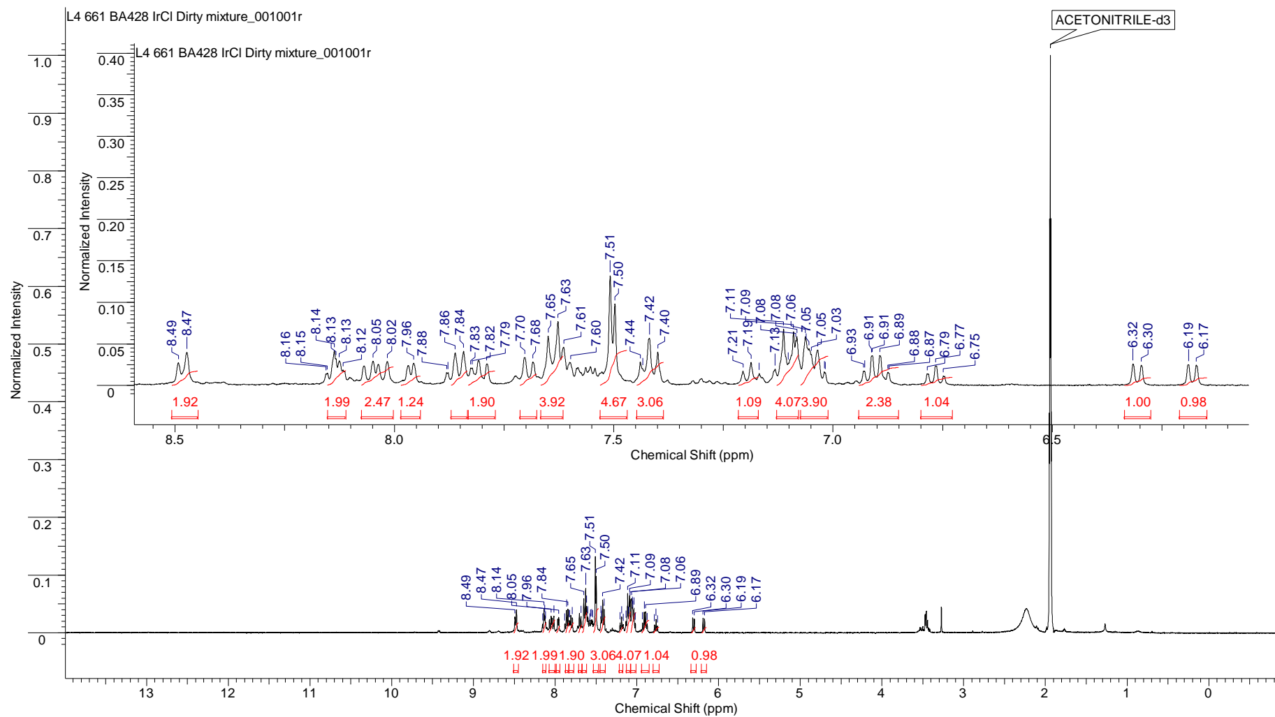
Figure S3 1 H NMR of the Irppy 2 L 4 .
