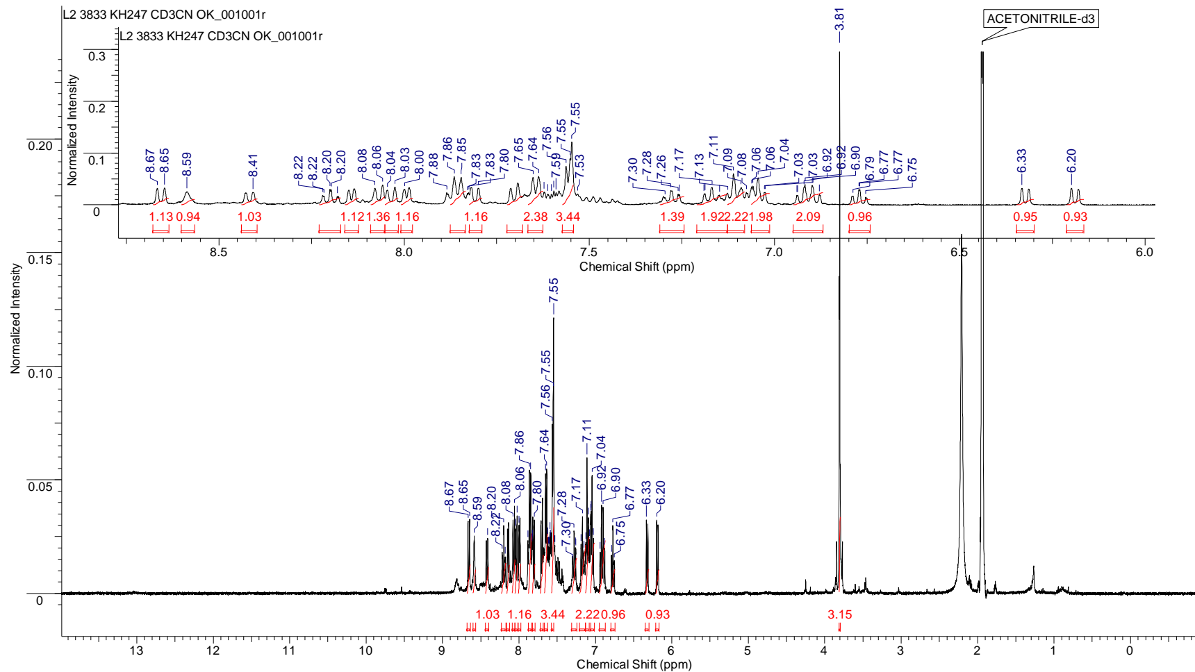
Figure S2 ^1\text{H} NMR of the Irppy 2 L 2 .
