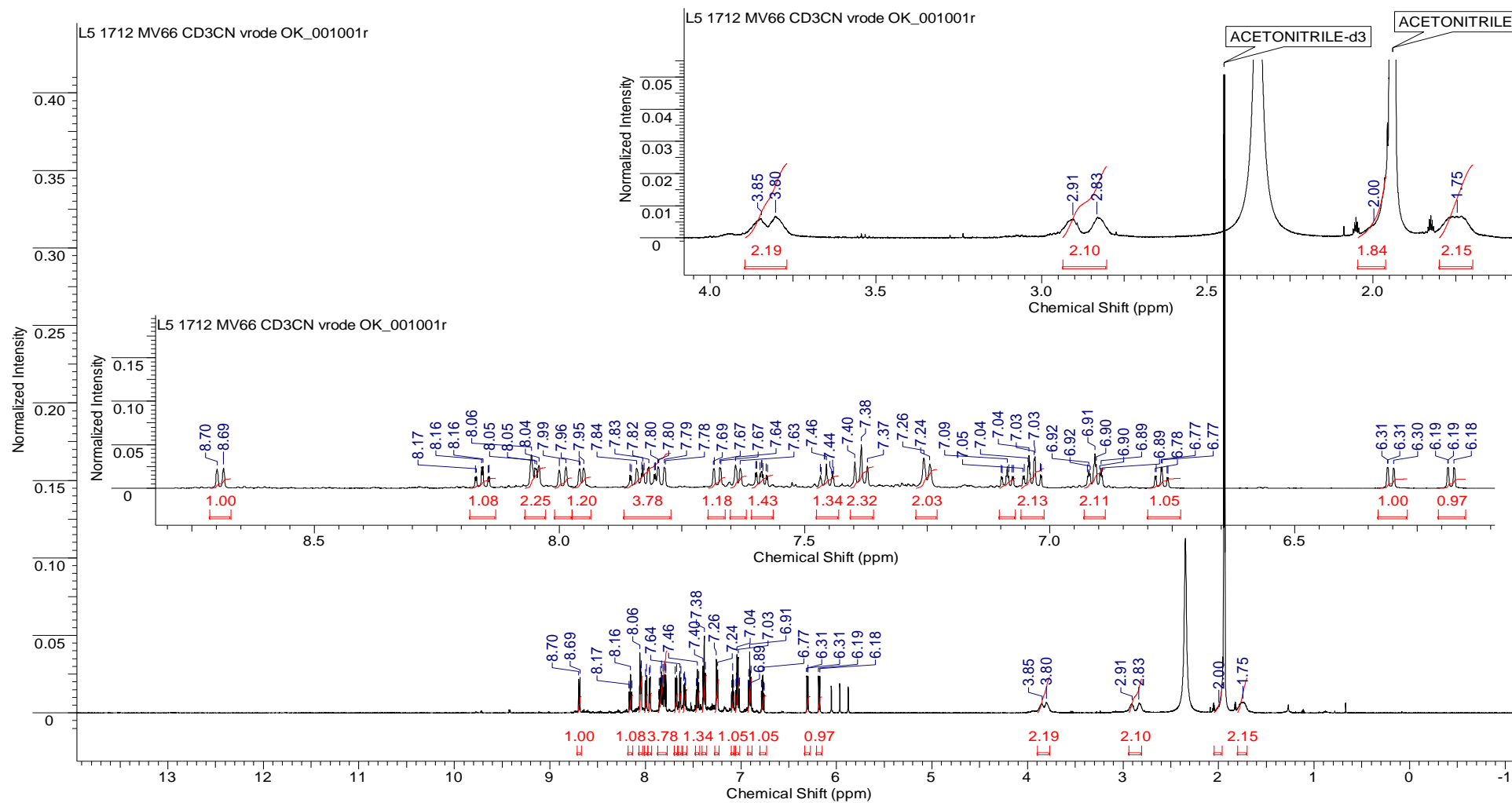
Figure S4 ^1\text{H} NMR of the Irppy 2 L5.
