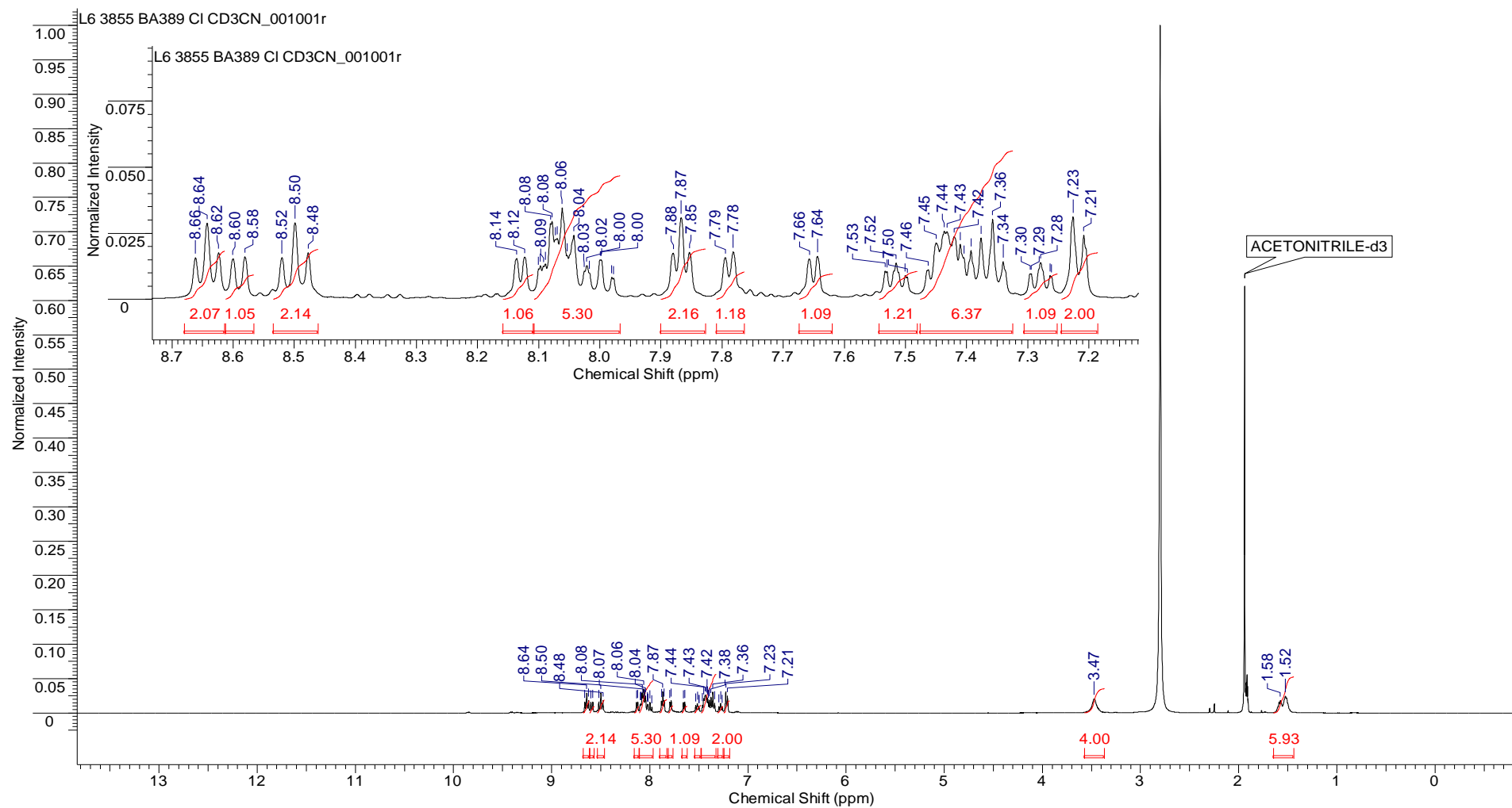
Figure S5 ^1\text{H} NMR of the Irppy 2 L6.
