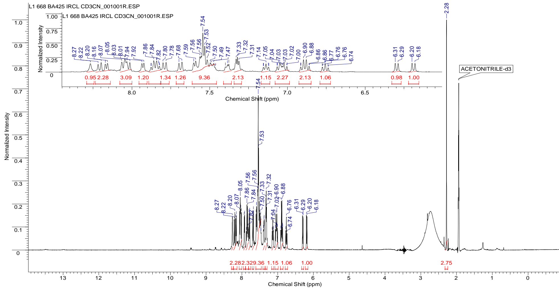
Figure S1 1 H NMR of the Irppy 2 L1.
