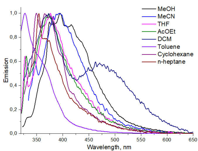
Figure 11 Emission spectra of compound 4a in various solvents.
